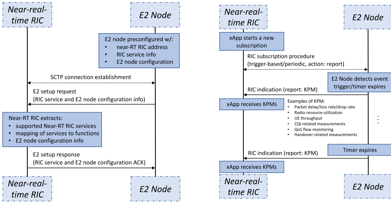
(a) Procedure for the setup of an E2 session between the near-RT RIC and an E2 node. The procedure is initiated by the E2 node which interacts with the near-RT RIC. (b) Procedures related to the streaming of KPMs from the E2 node to the near-RT RIC. The subscription procedure is started by an xApp on the near-RT RIC, which then receives the reports.
