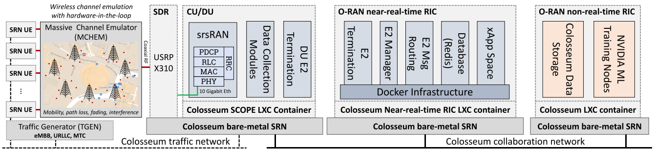
Fig. 16. OpenRAN Gym components [186] deployed on the Colosseum experimental testbed [187], adapted from [68]. The non-RT RIC, near-RT RIC, and RAN nodes (either base stations or users) are deployed as containers on different Colosseum Standard Radio Nodes (SRNs). Different Colosseum networks can be used to provide application traffic and support for the O-RAN interfaces, while the wireless communications among RAN components is emulated by the Massive Channel Emulator (MCHEM).
